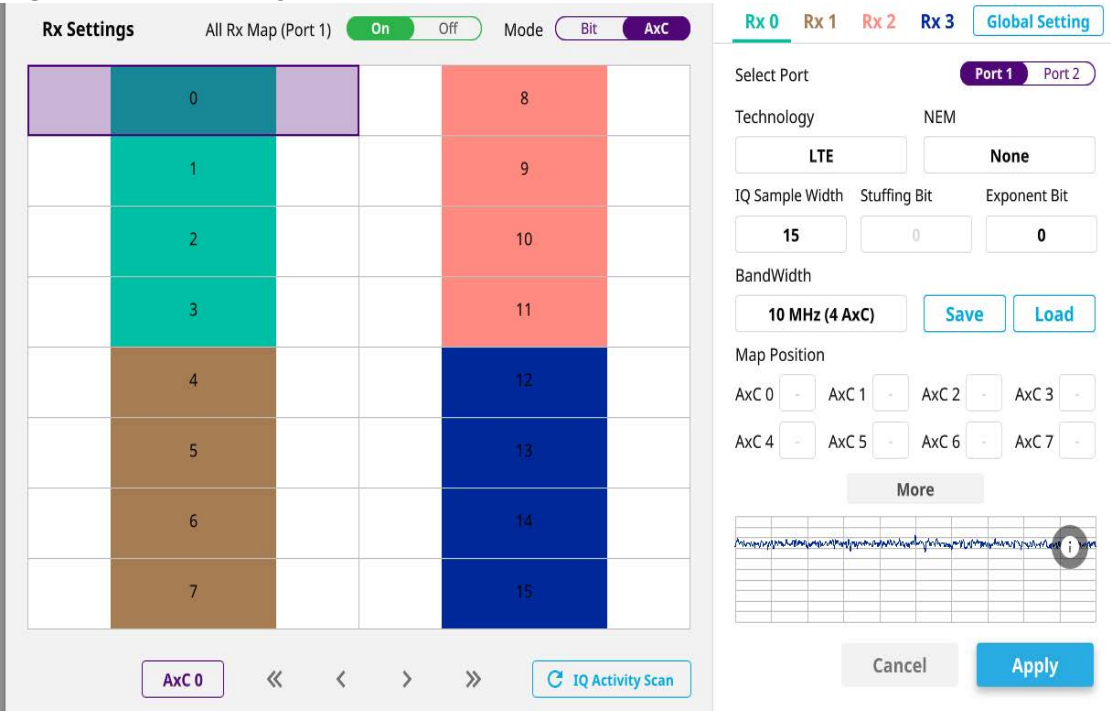
Figure 186 RX settings for AxC Mode
