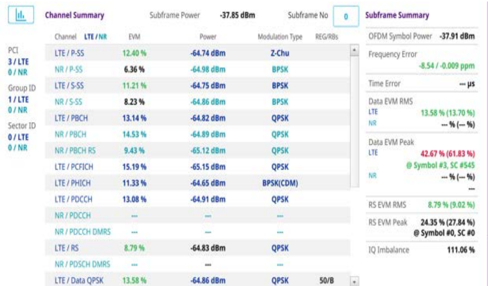
Figure 164 5G DSS DSS subframe measurement
