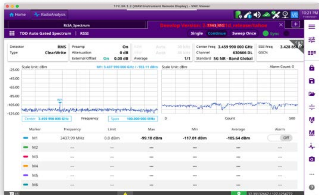
Figure 107 RSSI measurement
