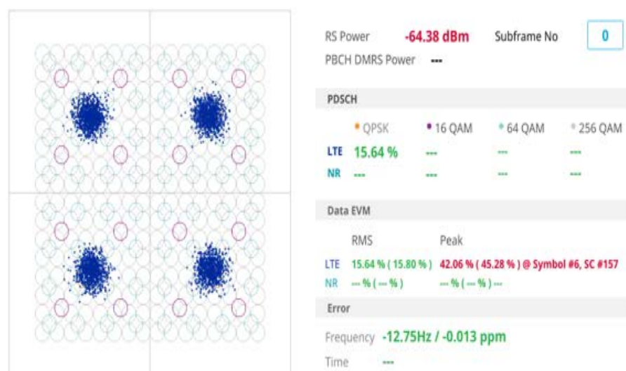
Figure 161 5G DSS DSS constellation measurement
