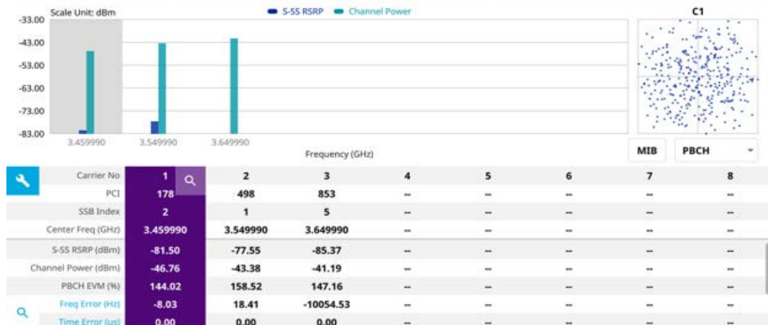
Figure 120 5G NR carrier scanner measurement
