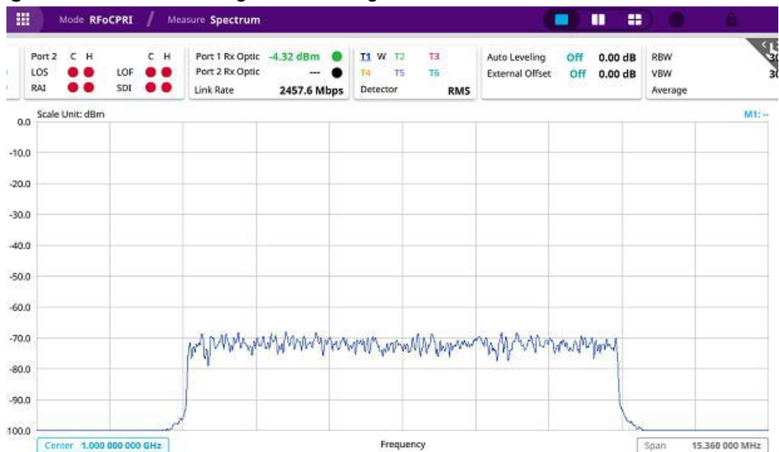
Figure 187 Before enabling Auto Leveling
