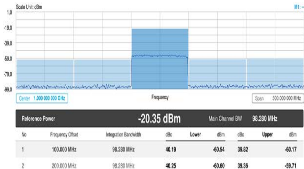
Figure 115 5G NR ACLR measurement
