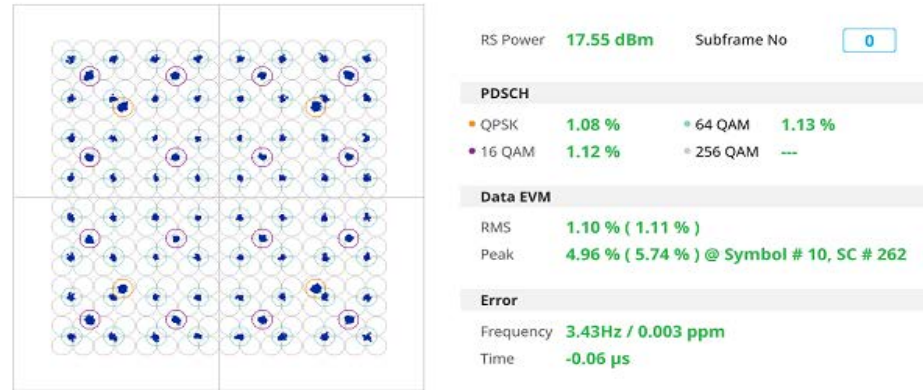
Figure 46 LTE/LTE-A FDD constellation measurement
