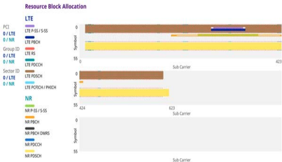
Figure 162 5G DSS DSS channel mapper measurement
