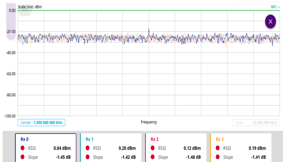
Figure 191 RFoCPRI PIM measurement
