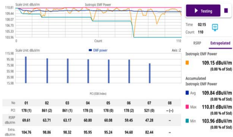
Figure 200 EMF 5G NR beam analyzer measurement (Extrapolated)
