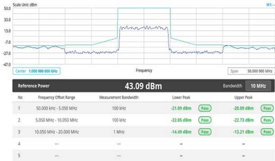
Figure 155 5G DSS spectrum emission mask measurement
