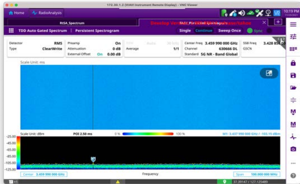
Figure 106 Persistent spectrogram measurement
