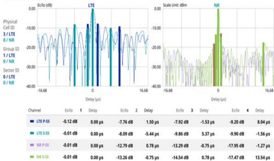
Figure 170 5G DSS OTA multipath profile measurement
