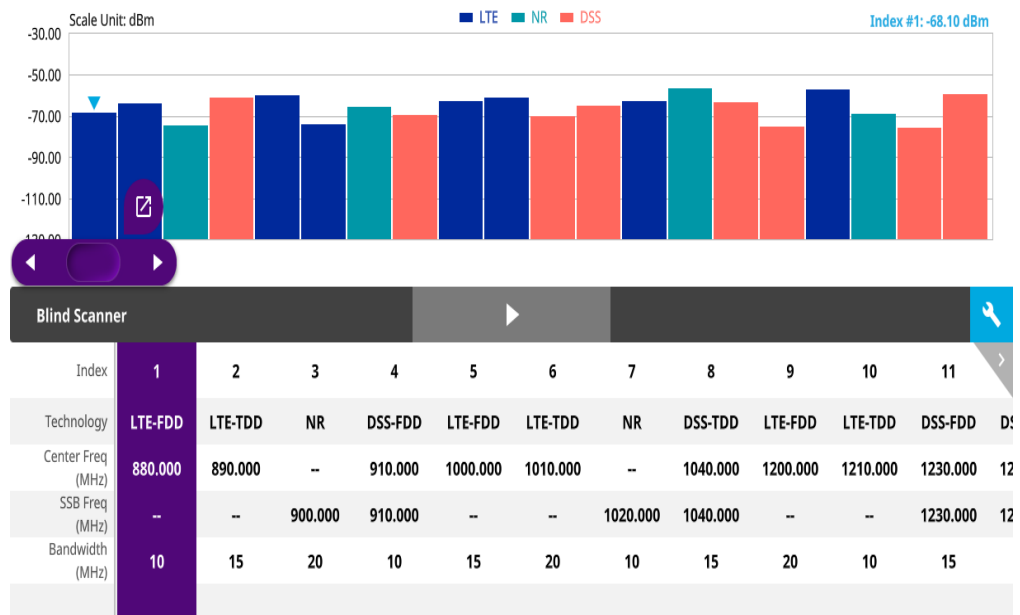
Figure 208 Blind Scan result
