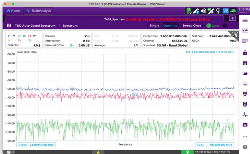
Figure 103 Specrum measurement with TAGS
