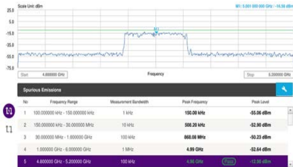
Figure 117 5G NR spurious emissions measurement
