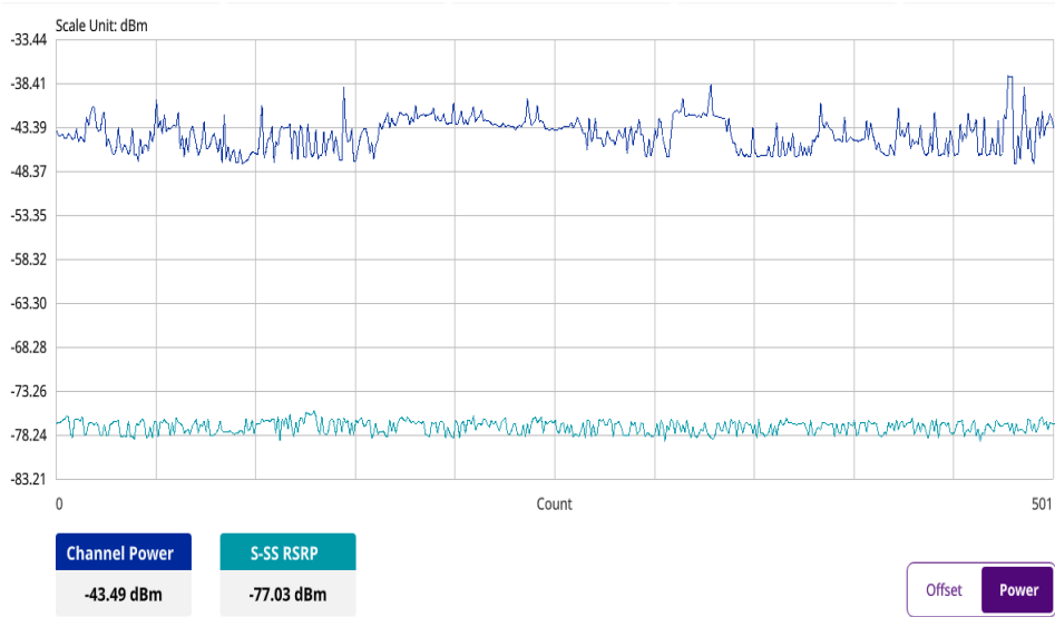
Figure 130 5G NR freq/time/power variation by power
