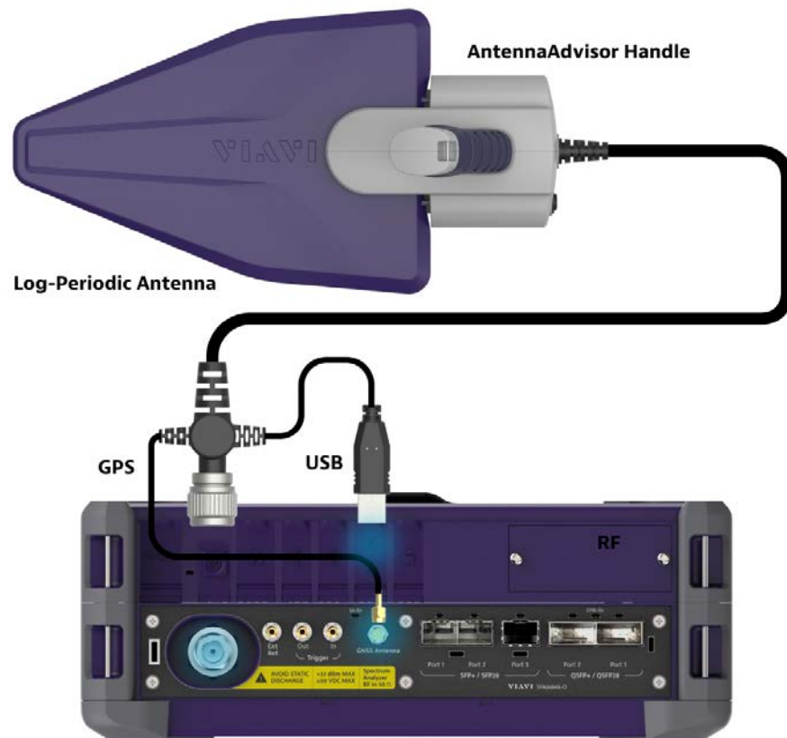
Figure 108 Antenna connection example
