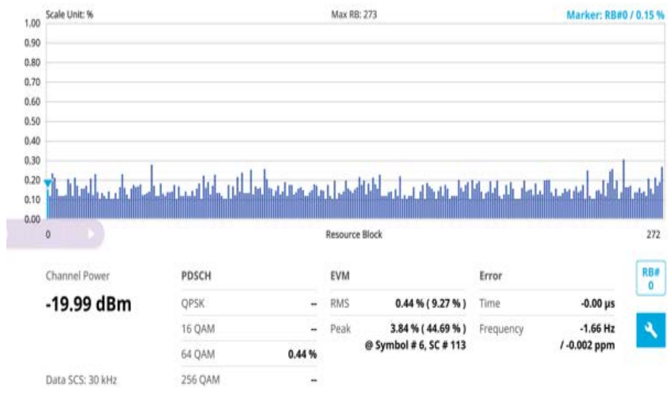
Figure 137 5G NR EVM vs subcarrier measurement
