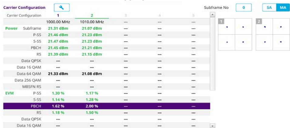
Figure 53 LTE/LTE-A FDD carrier aggregation measurement
