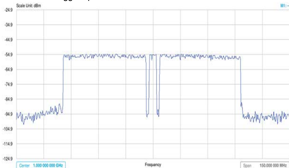
Figure 111 5G NR trigger spectrum measurement
