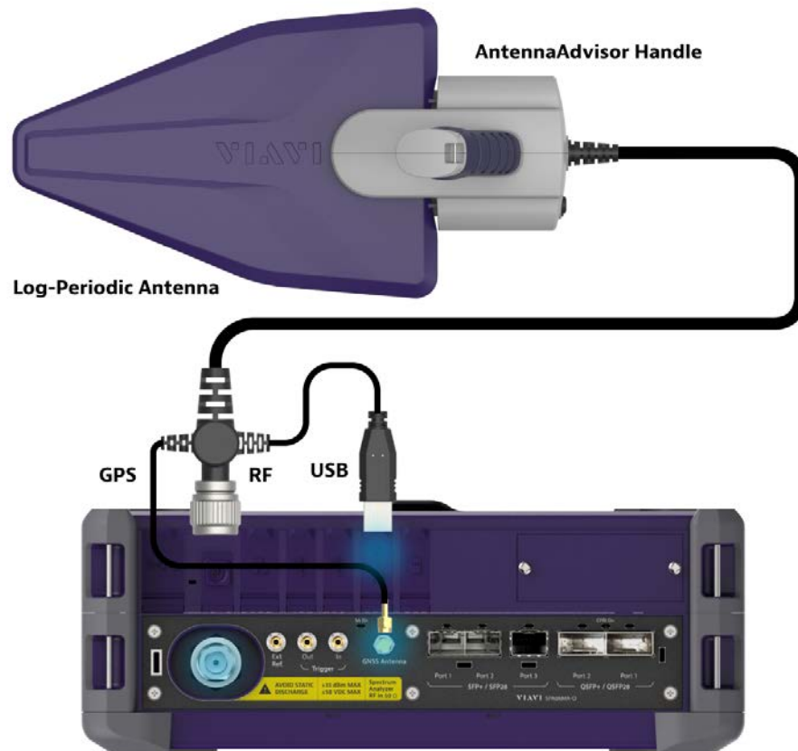
Figure 195 Connecting a log-periodic antenna
