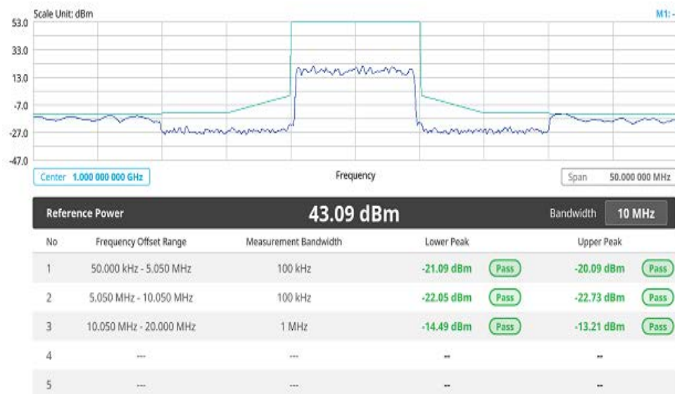
Figure 71 LTE/LTE-A TDD spectrum emission mask measurement
