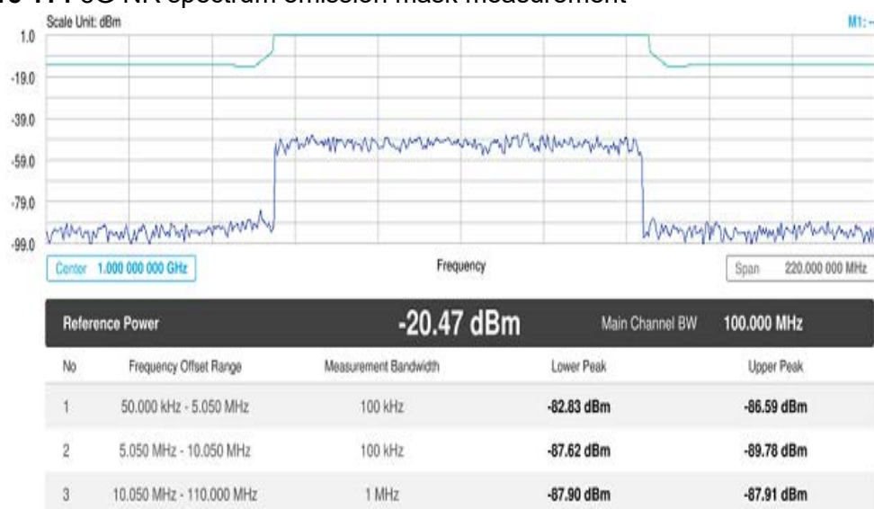
Figure 114 5G NR spectrum emission mask measurement
