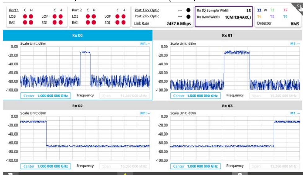
Figure 190 RFoCPRI spectrum measurement (Quad)
