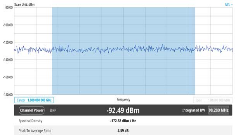
Figure 112 5G NR channel power measurement
