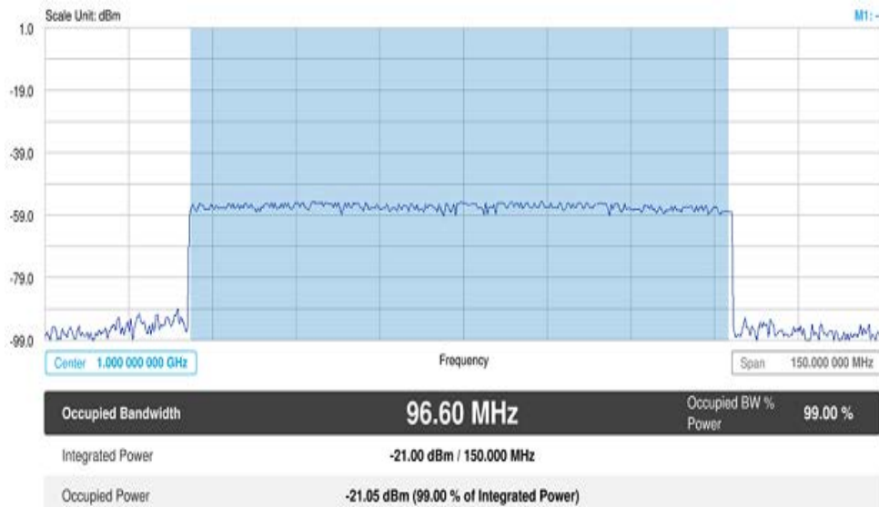
Figure 113 5G NR occupied bandwidth measurement
