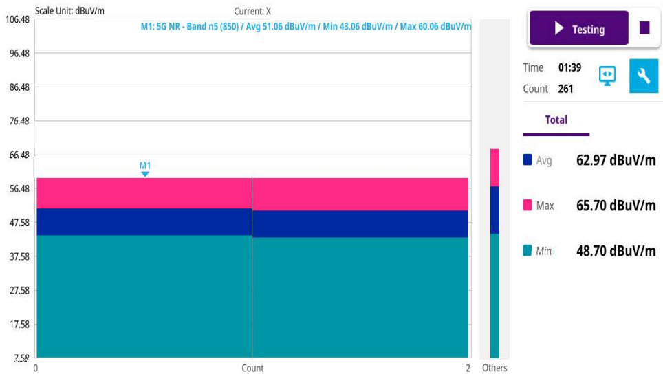
Figure 199 EMF scanner measurement
