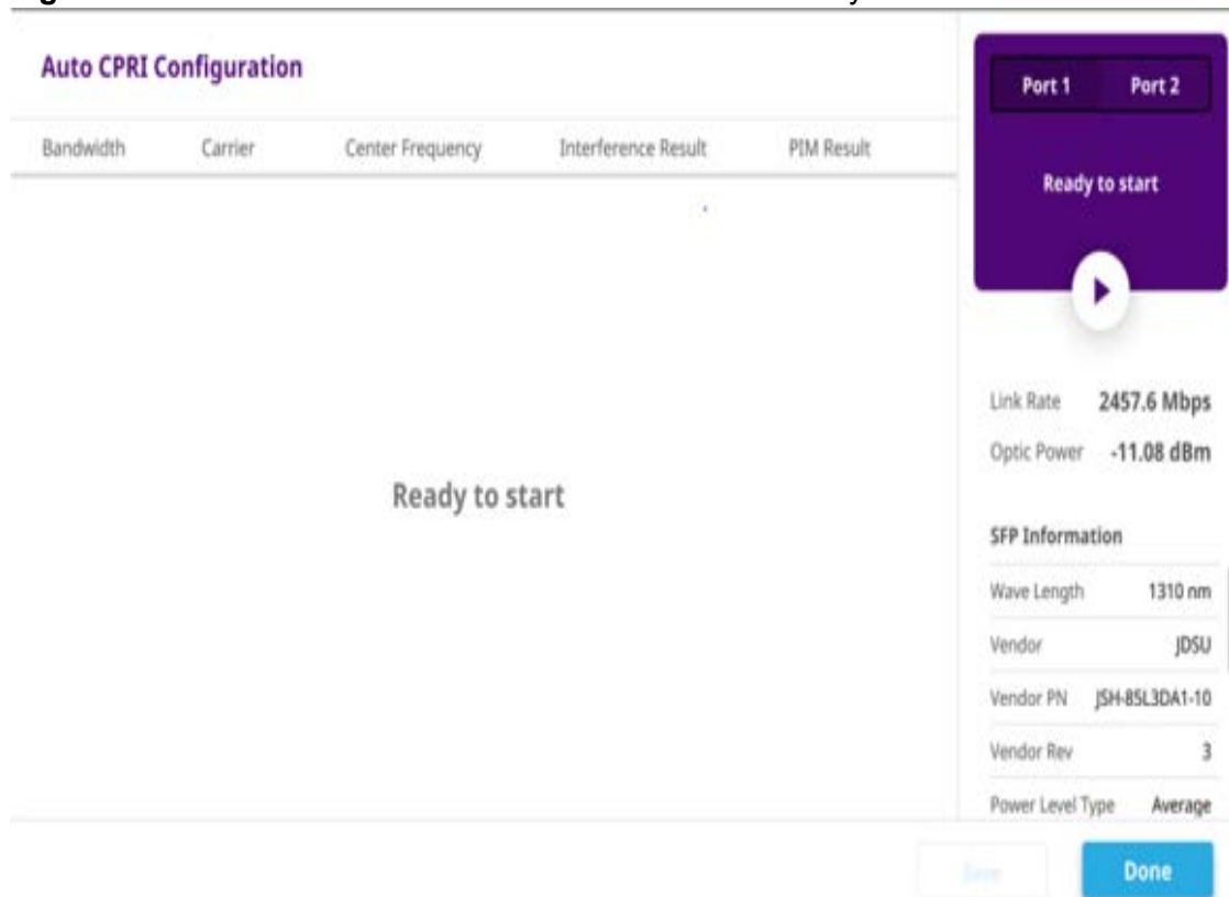
Figure 179 Carrier search with RFoCPRI Interference Analyzer
