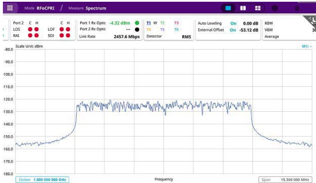
Figure 188 After enabling Auto Leveling
