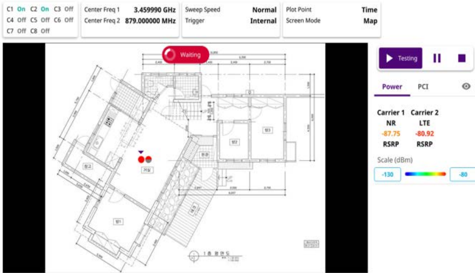
Figure 151 NSA route map measurement (Plot Point to Time)
