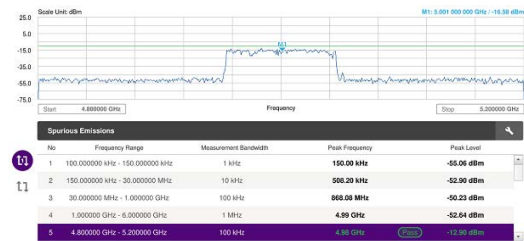
Figure 14 Spurious emissions measurement with spectrum analyzer
