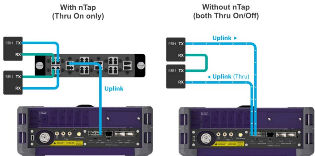
Figure 178 Connection diagram for interface analysis
