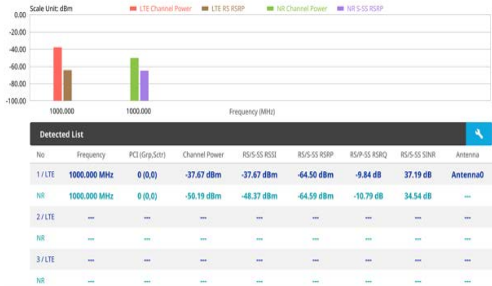
Figure 168 5G DSS OTA Channel Scanner measurement
