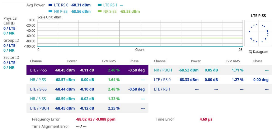
Figure 171 5G DSS OTA Control Channel measurement
