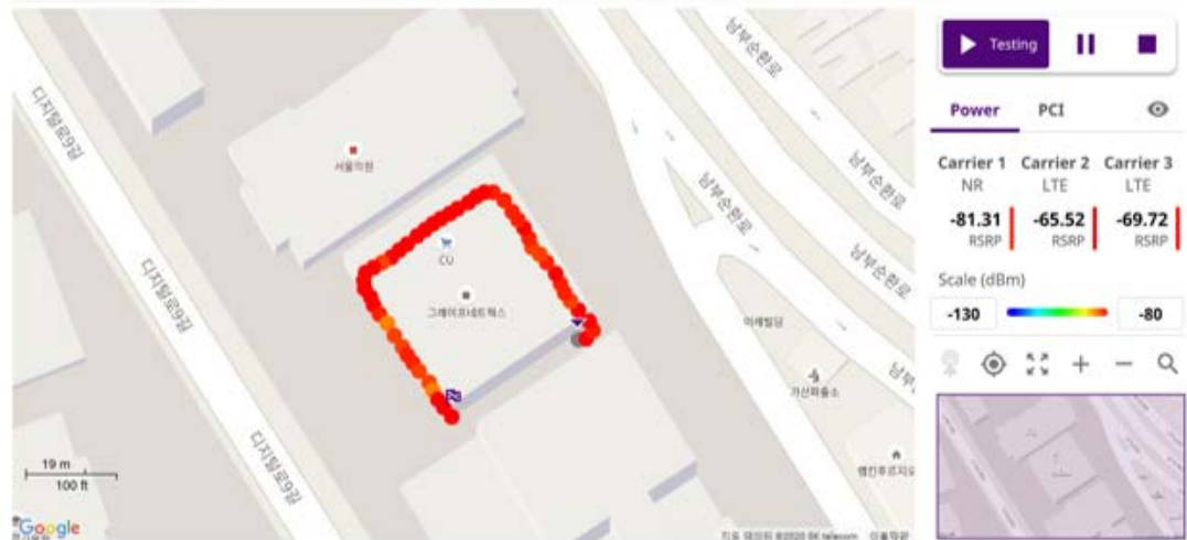
Figure 147 NSA route map measurement
