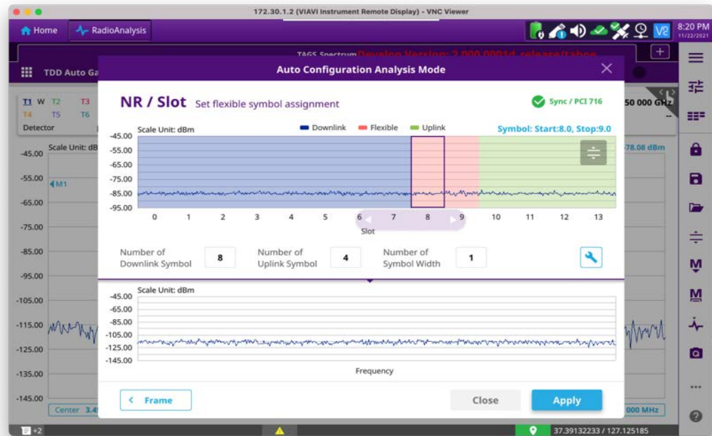
Figure 101 Slot format
