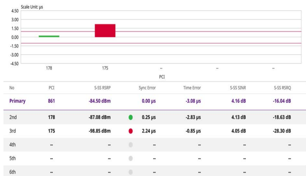
Figure 140 5G NR Sync Analysis measurement
