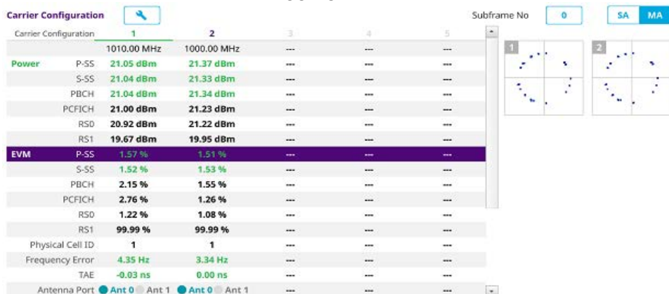
Figure 83 LTE/LTE-A TDD carrier aggregation measurement
