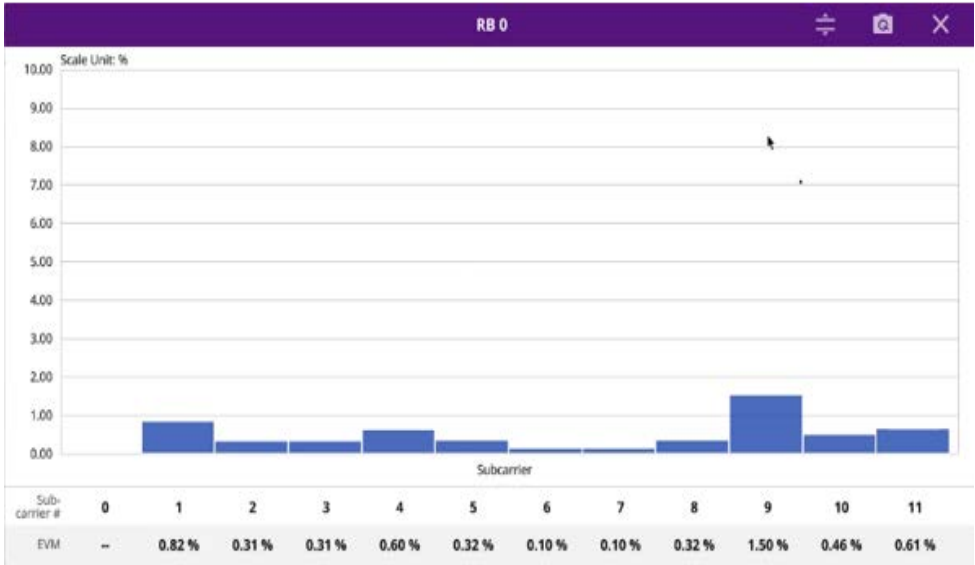
Figure 138 5G NR selected RB's EVM vs subcarrier measurement
