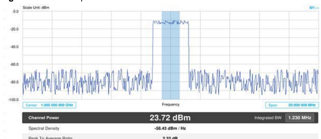
Figure 7 Channel power measurement
