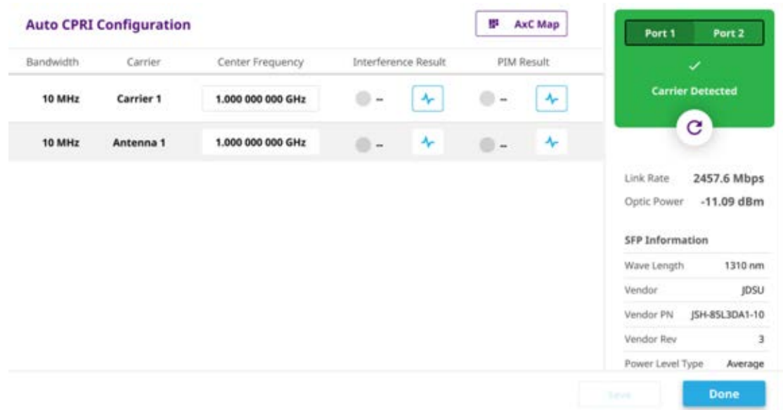
Figure 180 Detected carrier list with RFoCPRI Interference Analyzer
