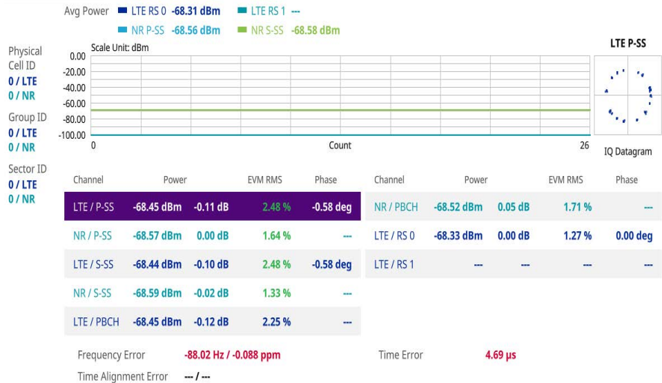
Figure 163 5G DSS DSS control channel measurement
