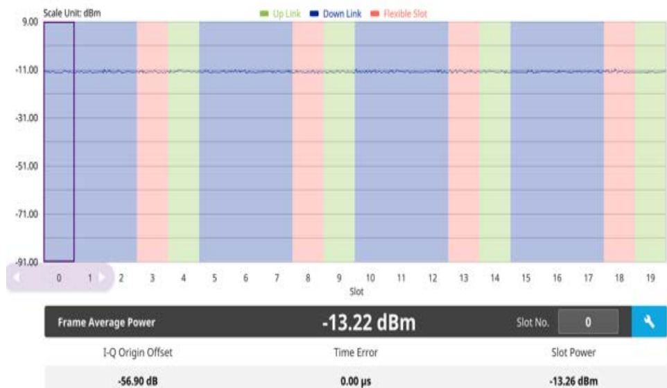
Figure 134 5G NR power vs time (frame) measurement
