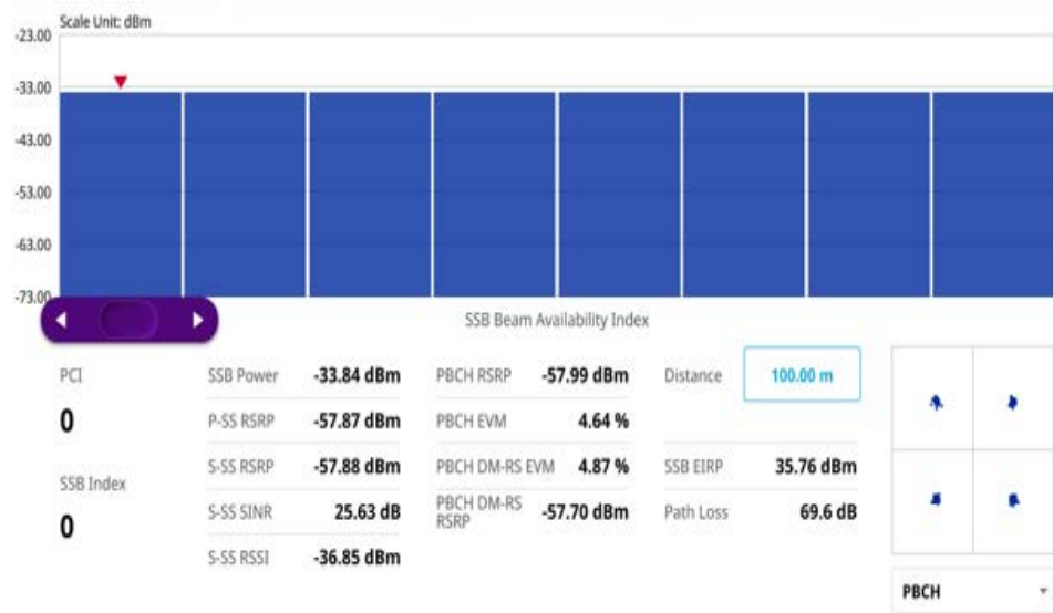
Figure 128 5G NR beam availability index
