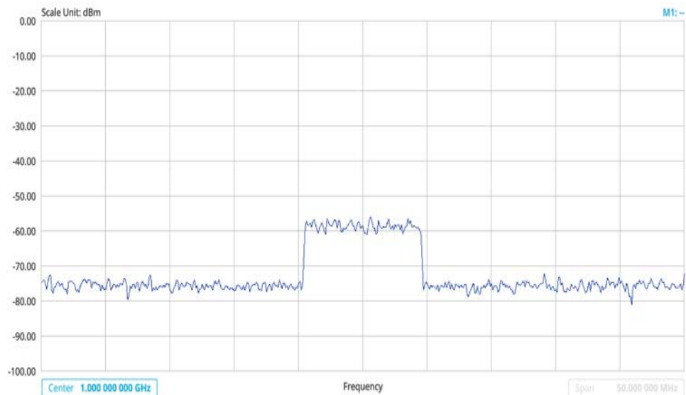
Figure 152 5G DSS spectrum measurement
