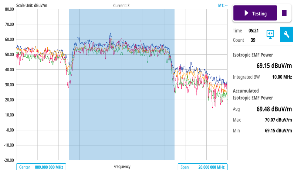
Figure 197 EMF spectrum (level recorder) measurement
