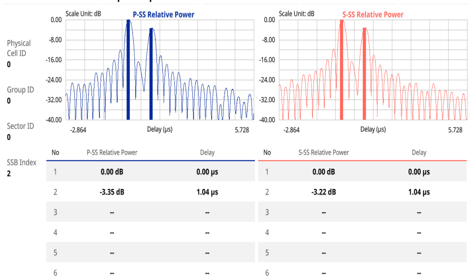
Figure 131 5G NR multipath profile
