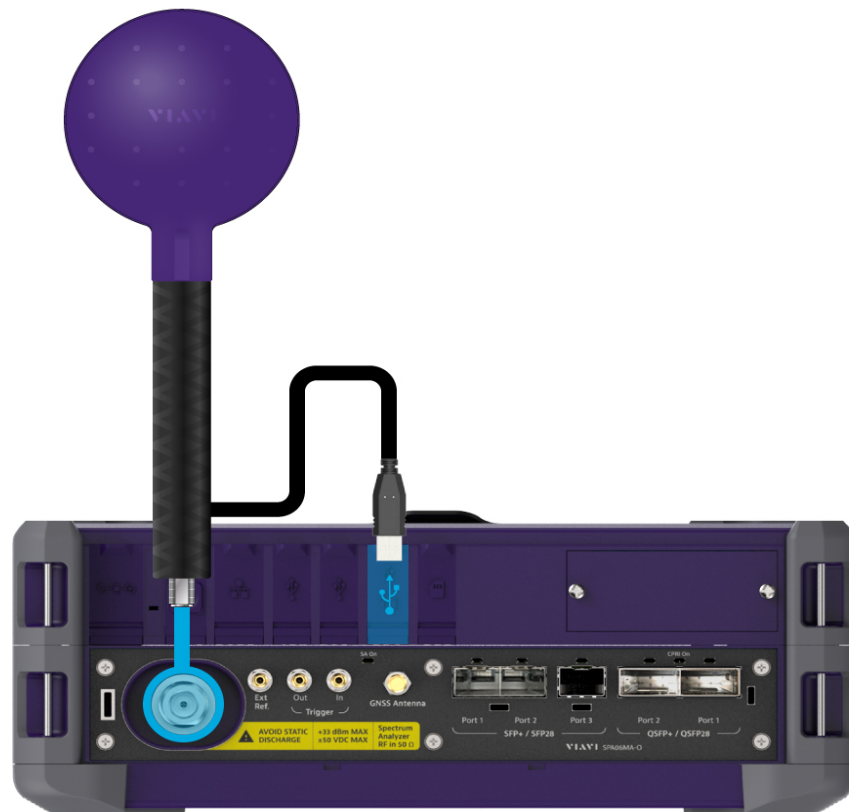
Figure 194 Connecting an isotropic antenna
