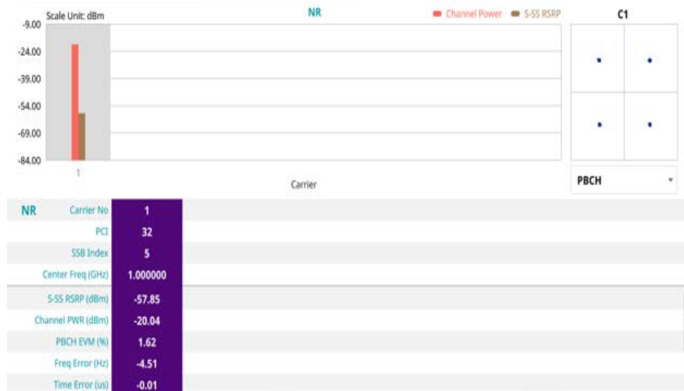
Figure 146 NSA scanner with only NR carrier measurement.
