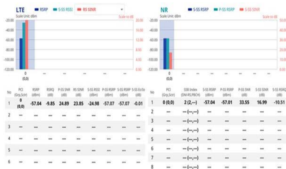
Figure 169 5G DSS OTA ID Scanner measurement
